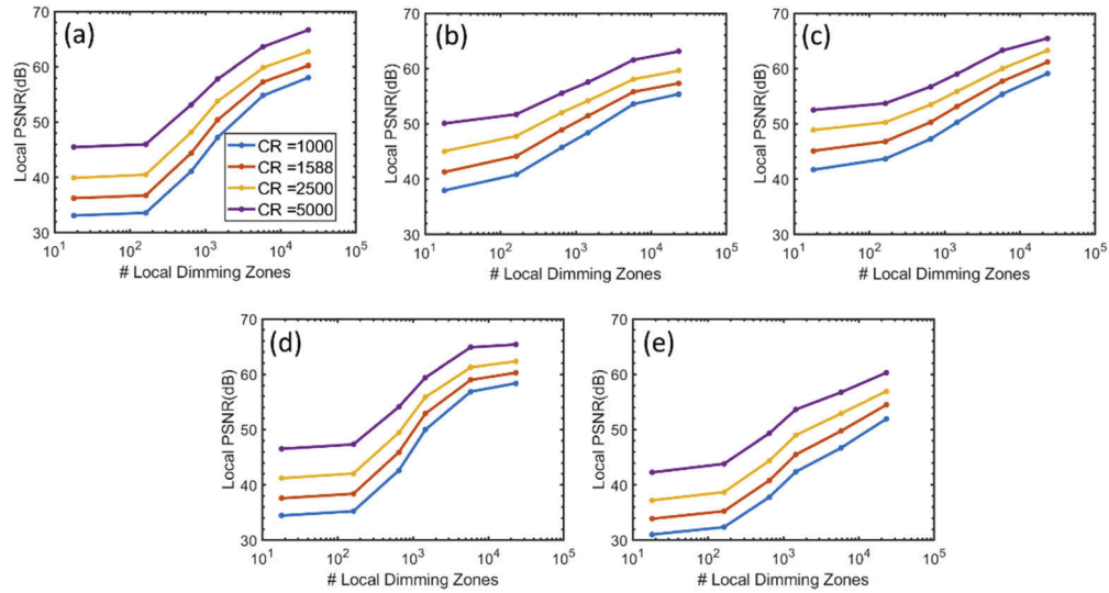
Fig. 10. Simulated LocalPSNR of target images under dark room: (a) Parking sign, (b) Ferris Wheel, (c) Mountains, (d) Chess, and (e) Tower.
