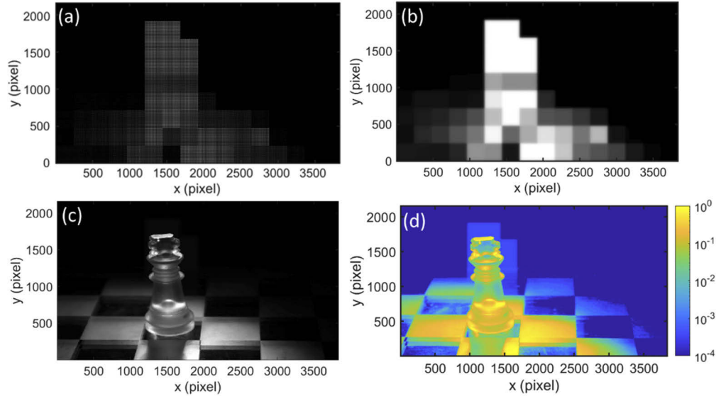
Fig. 1. Displayed image of a mLCD: (a) Intensity profile of the mini-LED backlight. (b) Luminance distribution of the light incident on LC layer. (c) Displayed image after LCD modulation. (d) Normalized contrast ratio distribution of the image displayed by mLCD.
