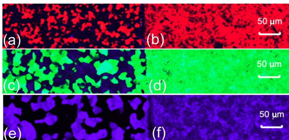
Figure 1. (a),(c),(e) Typical multi-domain blue phase platelet texture (b),(d),(e) monodomain blue phase texture with different pitch length. Reflective images. [Color figure can be viewed in the online issue, which is available at wileyonlinelibrary.com .]
