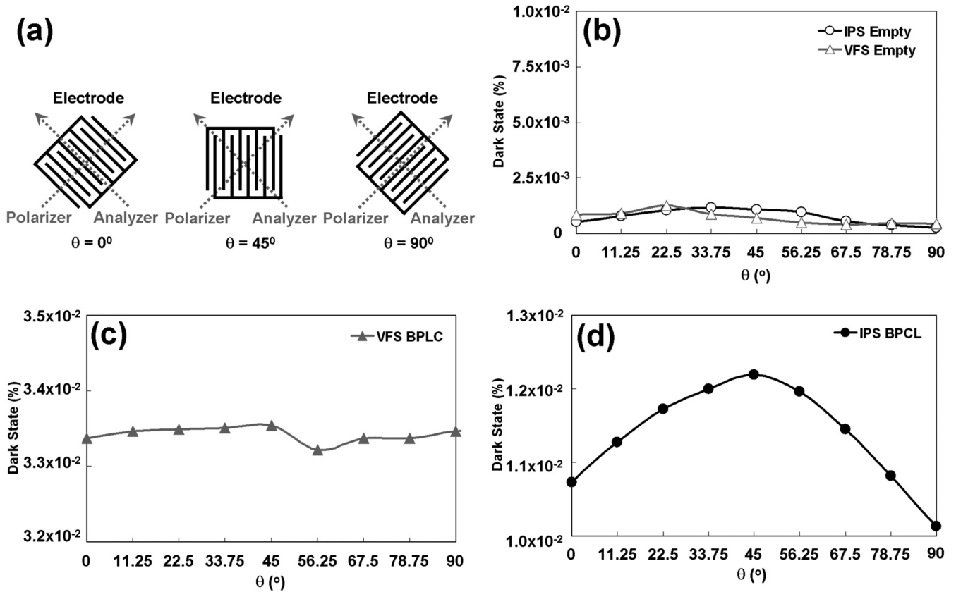
FIG. 1. Measurement of dark state by laser-detector system: (a) Definition of angle between transmittance axis of analyzer and electrode axis; (b) dark state of empty cell; (c) dark state of VFS BPLC cell, and (d) dark state of IPS BPLC cell.
