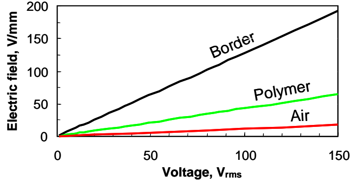
Fig. 2. Electric field within the LC layer at the lens border and lens center with various voltages applied across the electrodes. The LC cell gap is 25\ \mu\text{m} and the sag of the glass shell is 0.72\ \text{mm} . The filled material is either polymer NOA81 or air.
