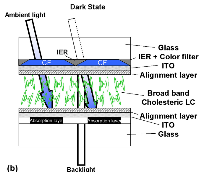
FIGURE 2 — Schematic plot of the proposed full-color transfective cholesteric LCD with an IER and wideband reflective cholesteric liquid crystal. (a) Bright and (b) dark state.
