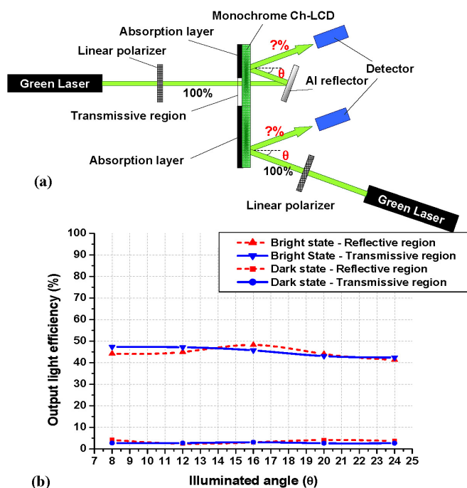
FIGURE 6 — (a) The experimental setup and (b) the measured output light efficiency of the IER function for a Ch-LCD.
