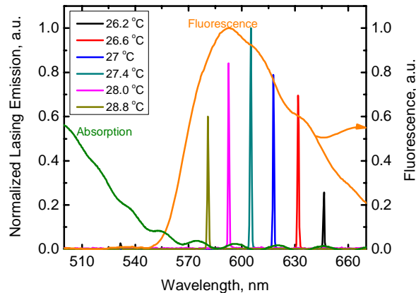
Fig. 6. Temperature dependent (normalized) laser emission wavelength. The CLC sample consists of 34 wt% ZLI-811 in BL-006 host, plus 1 wt% DCM dye. The pumping laser wavelength is \lambda=532 \text{ nm} .
