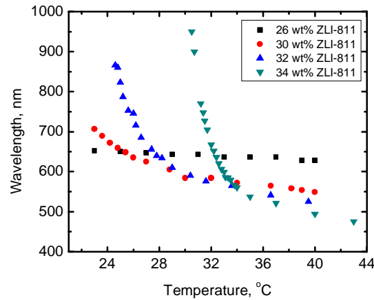
Fig. 3. The temperature dependent central wavelength of the CLC PBG.
