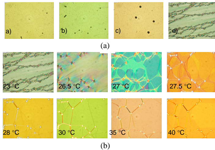
Fig. 4. (a) The microscope photos of the CLCs with different chiral dopant ZLI-811 concentrations: a) 24 wt%, b) 28 wt%, c) 32 wt%, and d) 34 wt%; (b) the microscope photos of the CLCs with 34 wt% chiral dopant ZLI-811 at different temperature.
