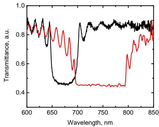
Fig. 1. The transmission spectra of the CLC cells mixed with 22 wt% ZLI-811 in BL006 (red line) and ZLI-4608 (black line) hosts, respectively.
