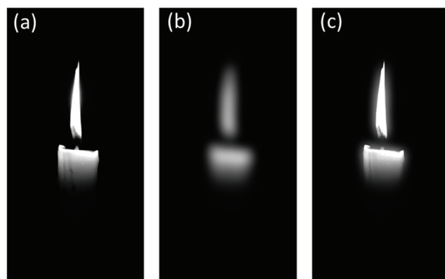
Fig. 4. Simulated intensity distribution of (a) without Gaussian filter, (b) with Gaussian filter at \rho = 3\text{mm} , and (c) our newly proposed method.
