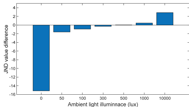
Fig. 10. Simulated average JND value difference between OLED and mini-LED backlit LCD at different ambient light illuminance.
