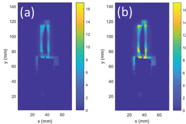
Fig. 8. JND between OLED display and mini-LED LCD at (a) 4% and (b) 1.2% ambient reflectance. The ambient light illuminance is 100 lux.
