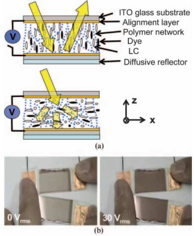
Figure 4. (a) Structure and operating principles of the dye-doped LC gel. (b) The dye-doped LC gel is trim-able (15).
