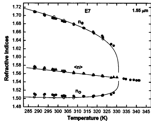
FIG. 4. Temperature-dependent refractive indices of E7 at \lambda=1.55 \mu\text{m} . The filled circles are the refractive indices n_e and n_o measured by the wedged LC cell method. The filled triangles are the average refractive index \langle n \rangle calculated by the experimental data. The open circles are the n_e and n_o extrapolated from the experimental data measured at visible spectrum using the extended Cauchy model. The open triangles are the average refractive index \langle n \rangle calculated by the extrapolated n_e and n_o . The solid curves are fittings using Eqs. (6a) and (6b). The solid straight line is the fitting using Eq. (5). The fitting parameters are listed in Table II.
