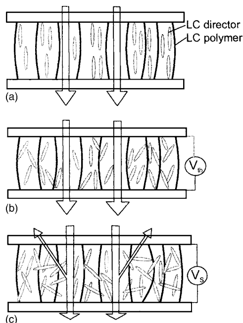
FIG. 1. Schematic diagrams of polymer and LC director orientations of a homeotropic LC gel: (a) V=0 , (b) V=V_{\text{th}} where the LC directors reorientation starts, and (c) V=V_s where the light scattering takes place.
